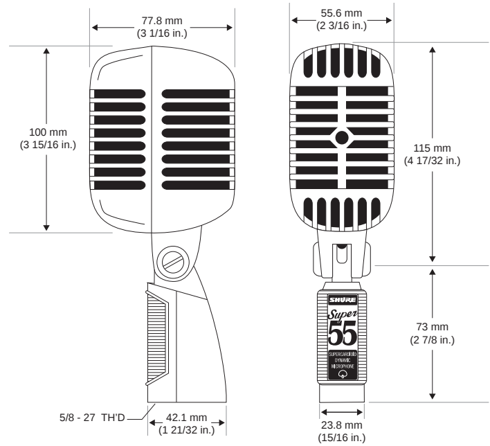
OVERALL DIMENSIONS
